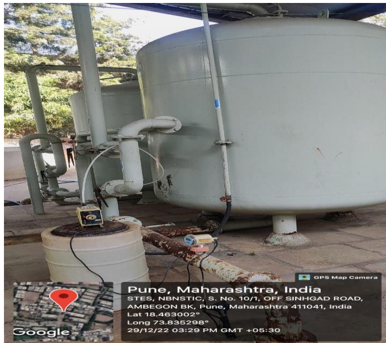
Fig. (A) Chlorine Dosing Pump
